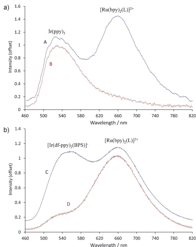
Figure 2. a) ECL spectra generated using an electrode sweep at 0.05 V s -1 from 0 to 1.04 V (spectrum A) or 0 to 0.44 V (spectrum B) vs. ferrocene for 0.5 mM [\text{Ir}(\text{ppy})_3] and 0.025 mM [\text{Ru}(\text{bpy})_2(\text{L})]^{2+} in acetonitrile/0.1 M TBAPF 6 (TBA = tetrabutylammonium) with 10 mM tripropylamine (TPA) as co-reactant. b) ECL spectra generated using chronoamperometry pulses at C) 1.30 V or D) 1.04 V vs. ferrocene for 0.1 mM [\text{Ir}(\text{df-ppy})_2(\text{BPS})]^- and 0.01 mM [\text{Ru}(\text{bpy})_2(\text{L})]^{2+} in 0.1 M phosphate buffer, 1:1 v/v water/acetonitrile with 10 mM TPA co-reactant (see the Supporting Information for further details).
