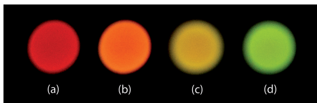
Figure 1. Photographs of electrogenerated chemiluminescence from a single solution of two metal complexes at four electrode potentials: a) 0.8 V, b) 0.95 V, c) 1.23 V, and d) 1.40 V (versus the ferrocene/ferrocenium couple). The solution contained 0.95 mM [\text{Ir}(\text{df-ppy})_2]^- (BPS) ^- and 0.05 mM [\text{Ru}(\text{bpy})_2(\text{L})]^{2+} (see Scheme 1 for chemical structures), with 30 mM TPA co-reactant, and 0.1 M phosphate buffer in 1:1 v/v water/acetonitrile. The colors were first observed by the naked eye, and then photographs were taken at values of applied potential that provided the greatest differences. Longer exposure times were used for the redder emissions to achieve uniform image brightness.
